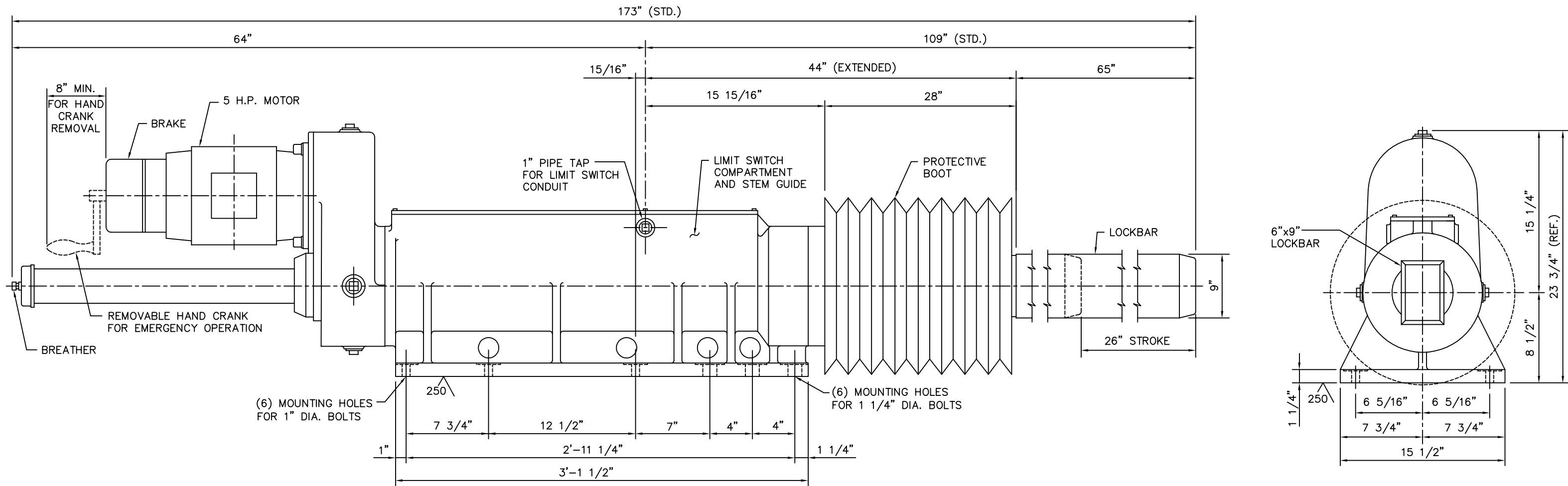
EARLE® EG-3 LOCKBAR OPERATOR
