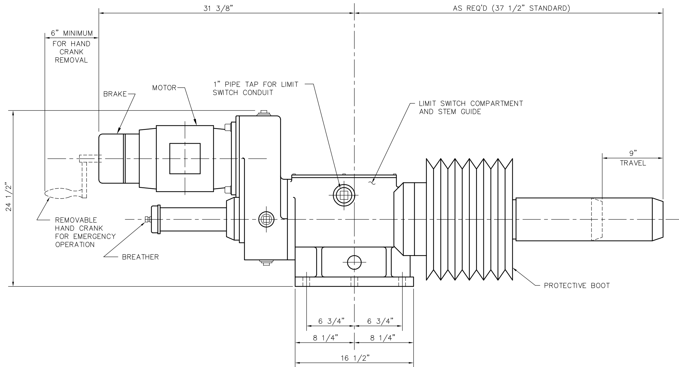
EARLE ® EG-2B LOCKBAR OPERATOR
